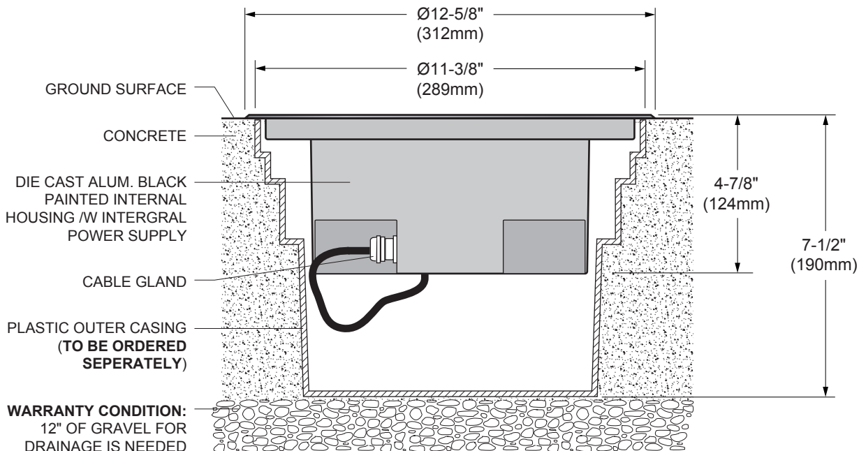
SECTION VIEW
