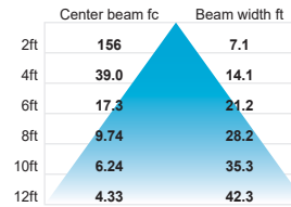
Illuminance at Distance
